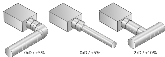
Figur 1. ROC + ALS.
