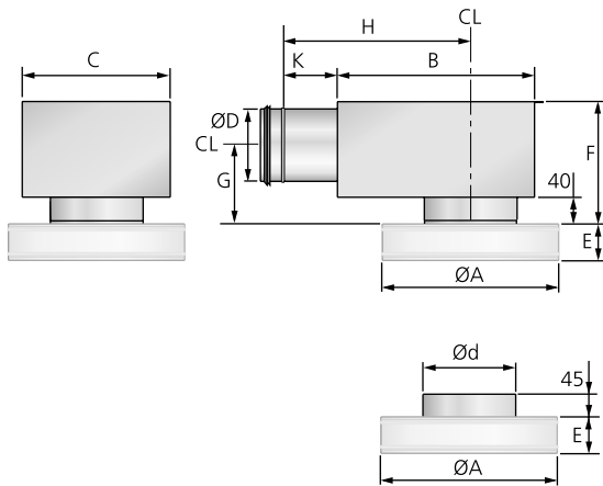
Figure 3. ROC + ALS.
