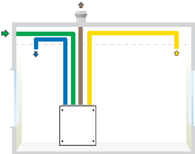
Duct connections on CASA R7.
