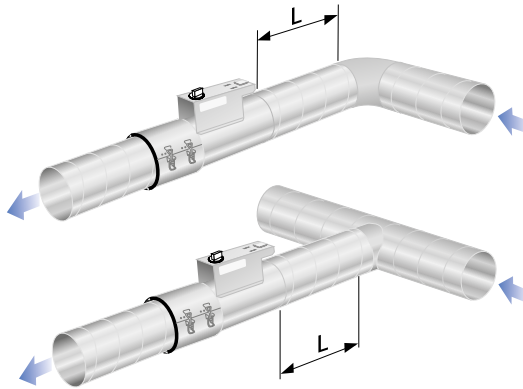
Figure 14. Straight duct length demands, see table below.
