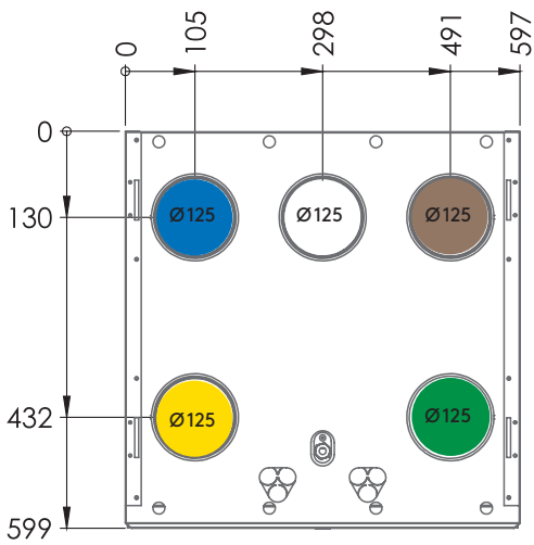
CASA W3 Smart XS R, right-hand version
