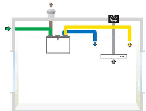
CASA W3 Smart XS L, duct connections and cooker hood connected to the external ceiling fan.
